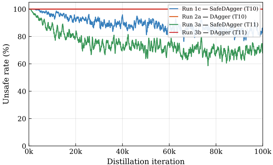
Student Unsafe Rate During Distillation (0-100k)
