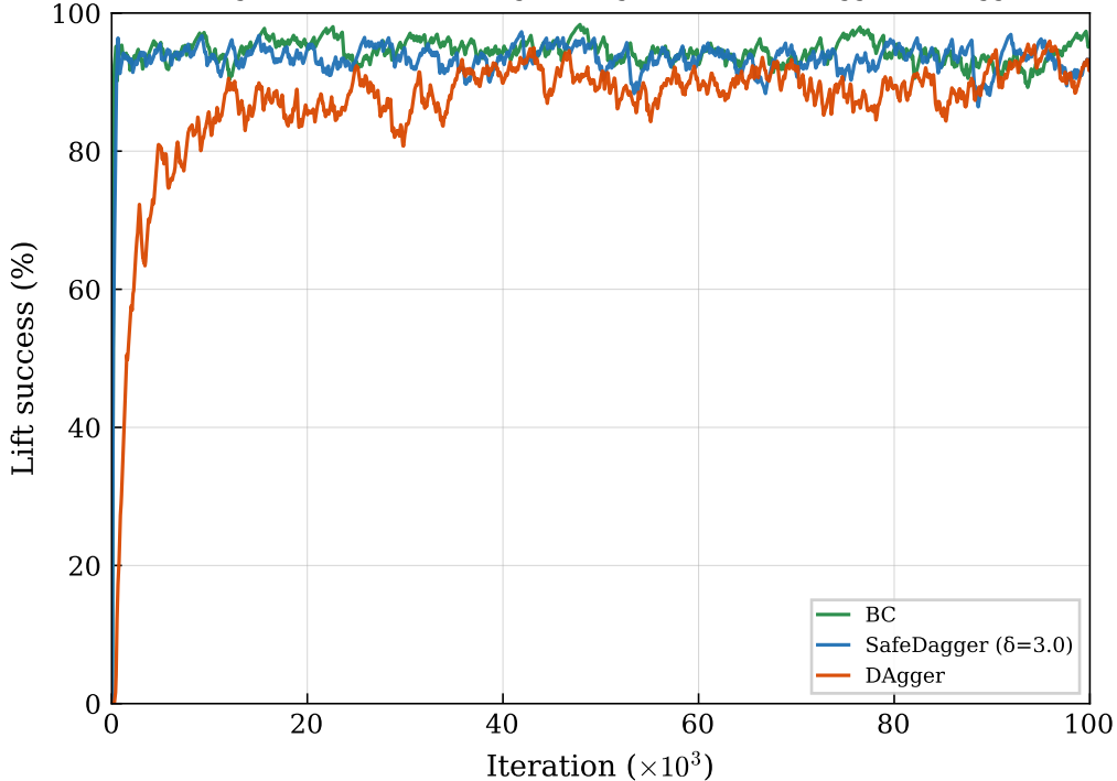
Hold-gated lift success during training — BC vs. SafeDagger vs. DAgger
