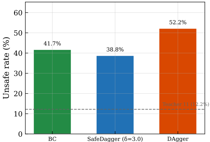
Unsafe episode rate — BC vs. SafeDagger vs. DAgger
