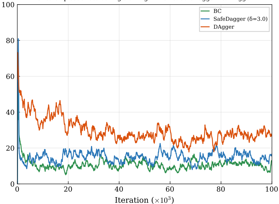
Unsafe episode rate during training — BC vs. SafeDagger vs. DAgger
