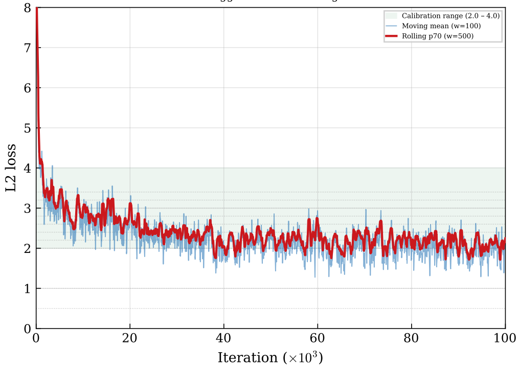
Dagger L2 over training
