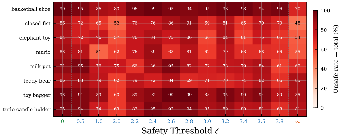
Run 14 — Per-object unsafe rate (incl. physics)
