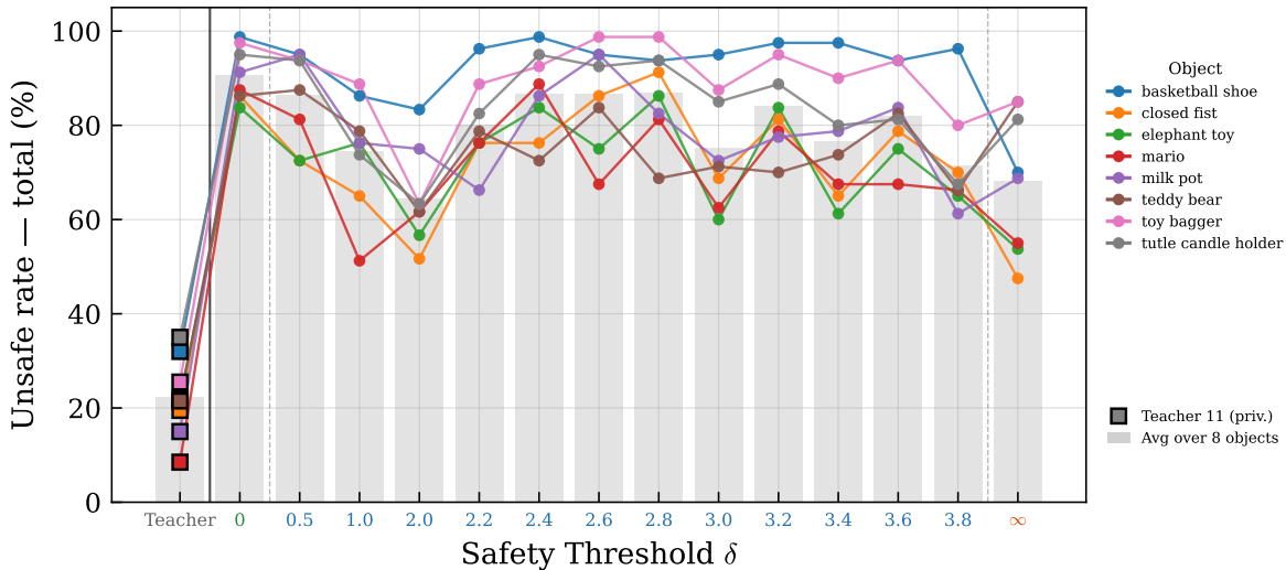
Run 14 — Per-object unsafe rate across threshold sweep (vs. Teacher 11) (incl. physics)
