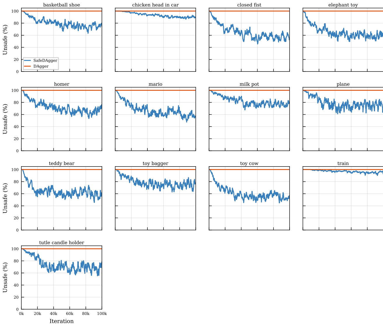
Per-Object Unsafe Rate: SafeDagger vs DAgger (0-100k)
