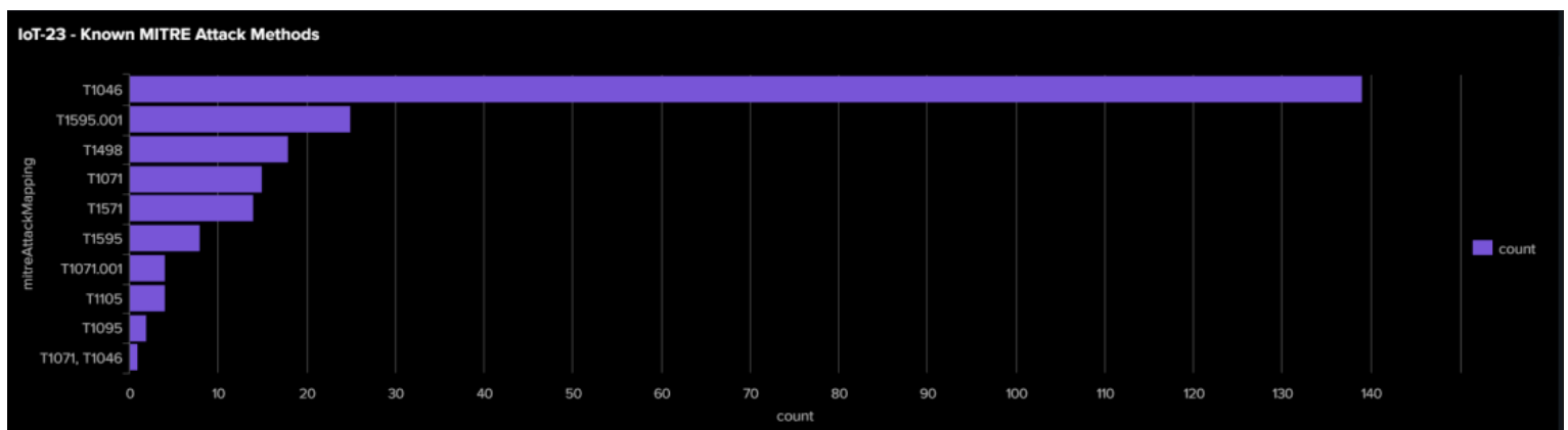
Fig 4 MITRE Attacks Identified by Gemini Pro
