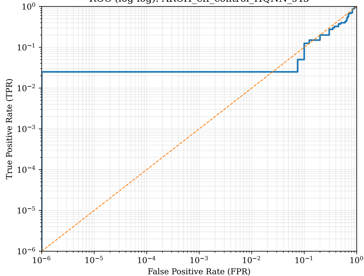
ROC (log-log): ARCH_eff_control_HQNN_s45
