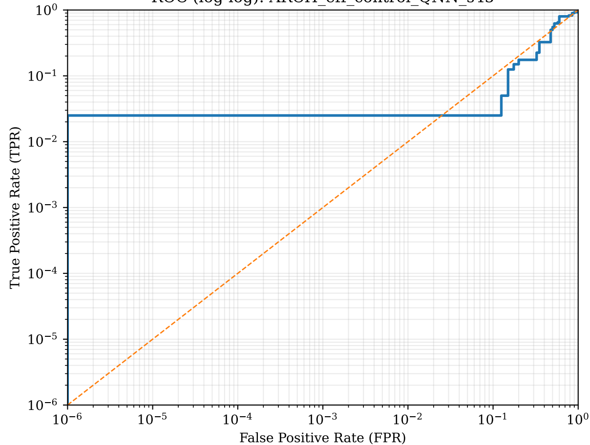
ROC (log-log): ARCH_eff_control_QNN_s45
