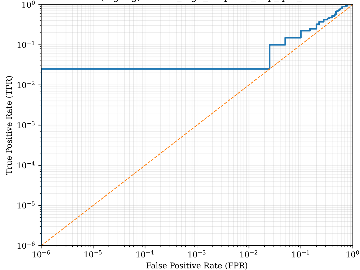
ROC (log-log): ARCH_high_reupload_mlp_qnn_s44
