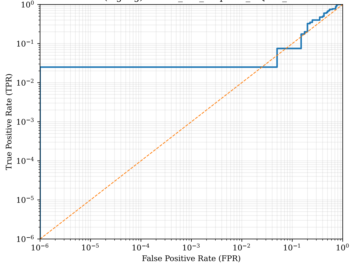
ROC (log-log): ARCH_low_reupload_HQNN_s43
