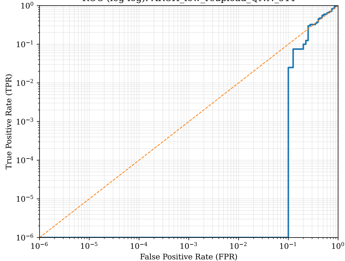
ROC (log-log): ARCH_low_reupload_QNN_s44
