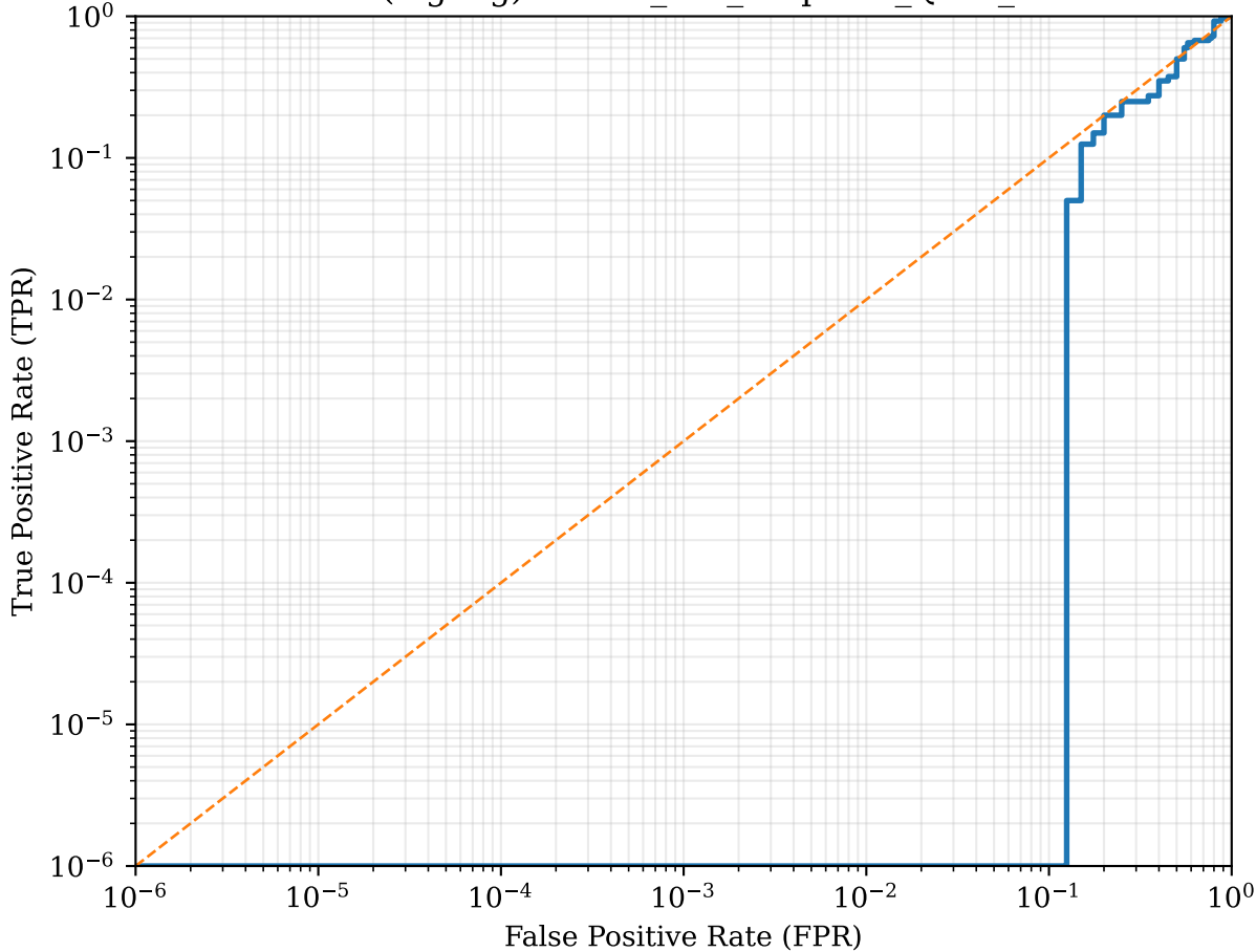
ROC (log-log): ARCH_low_reupload_QNN_s45
