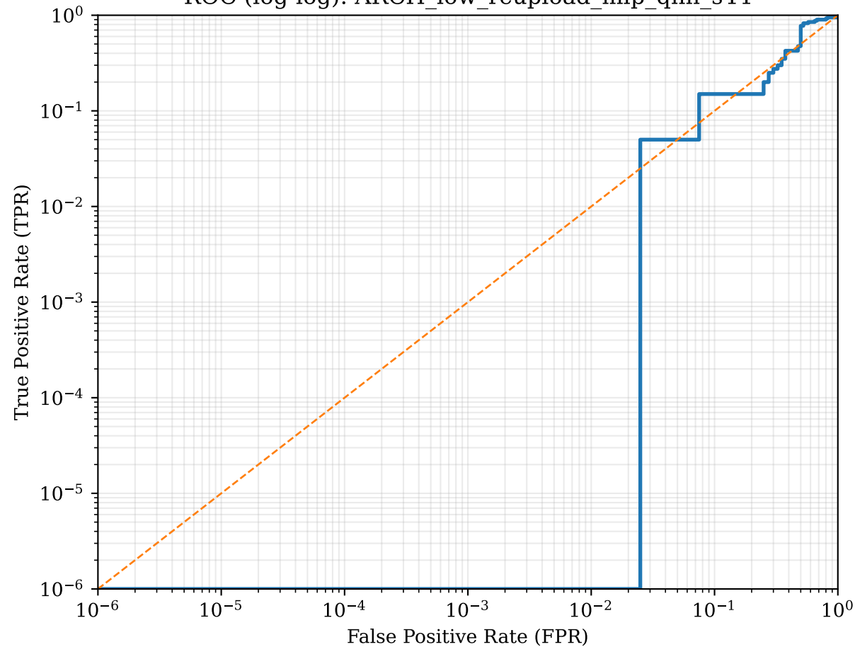
ROC (log-log): ARCH_low_reupload_mlp_qnn_s44
