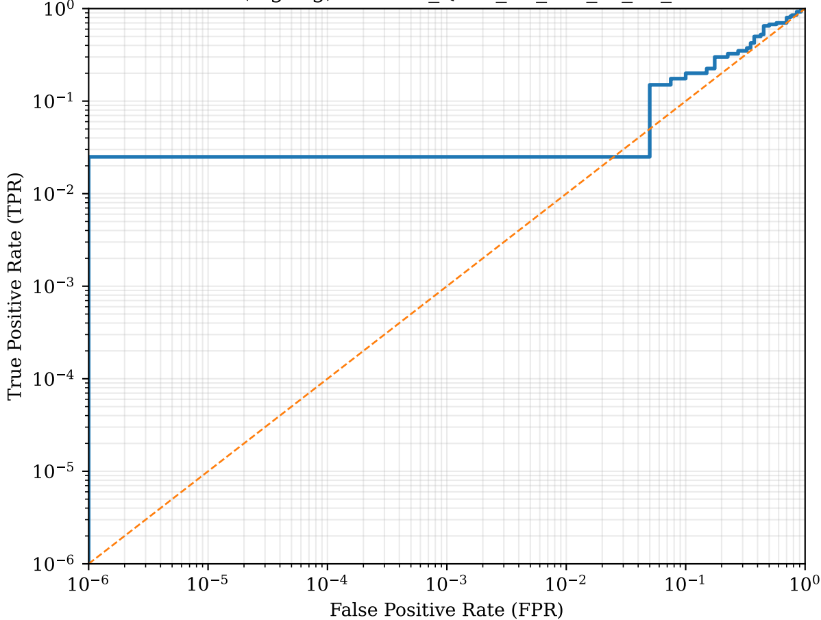
ROC (log-log): MNIST_QNN_eff_su2_r1_d2_s44
