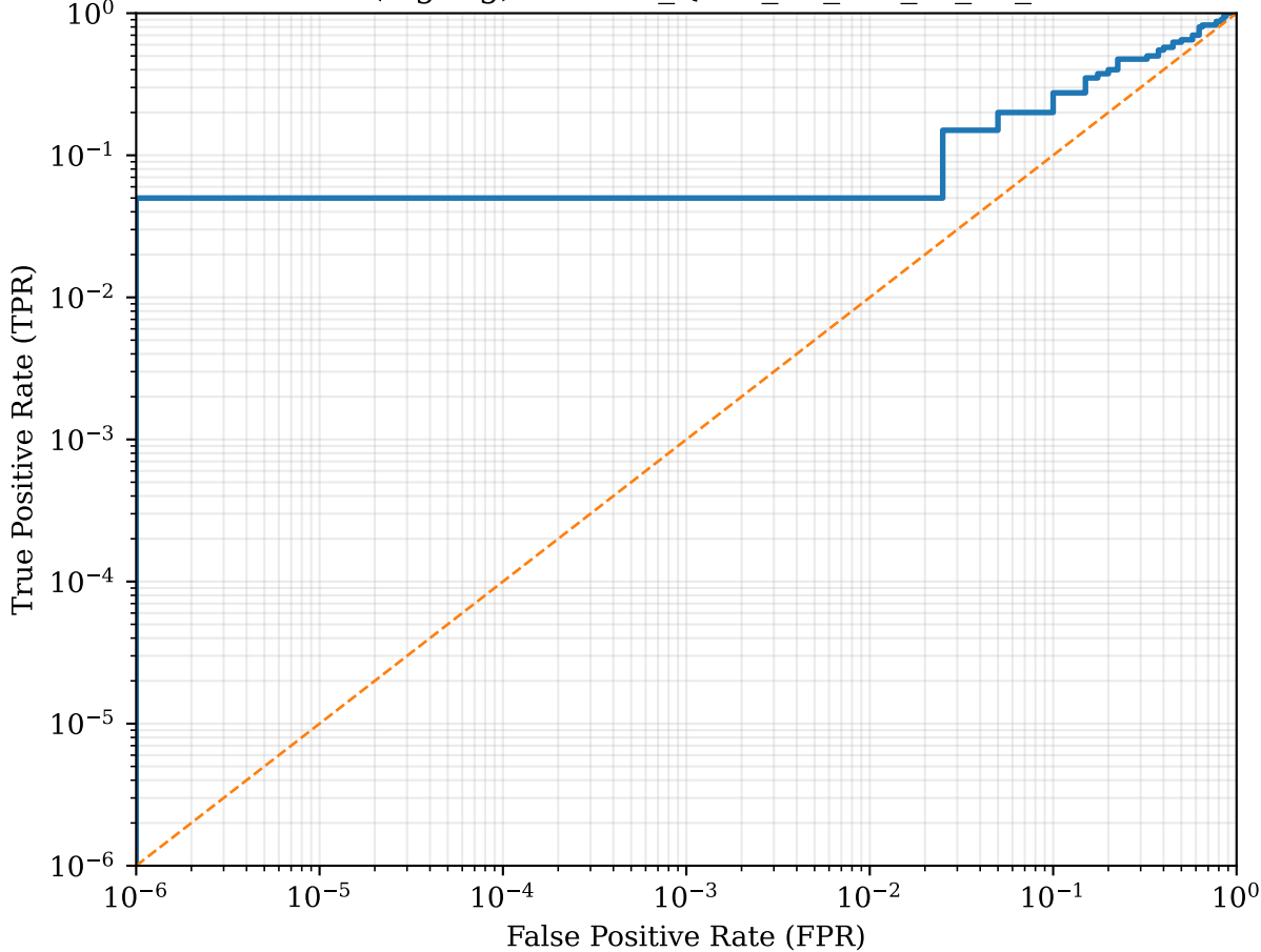
ROC (log-log): MNIST_QNN_eff_su2_r1_d2_s45
