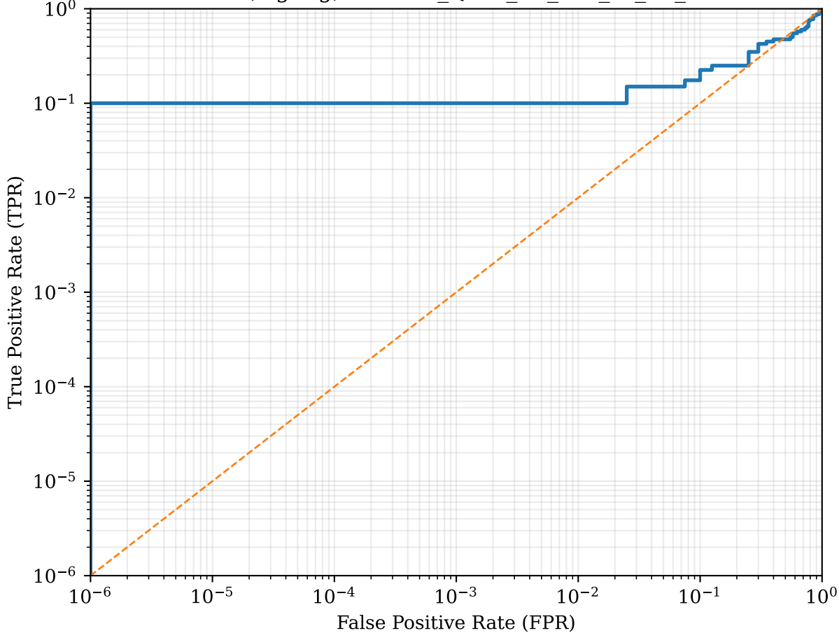
ROC (log-log): MNIST_QNN_eff_su2_r1_d6_s44
