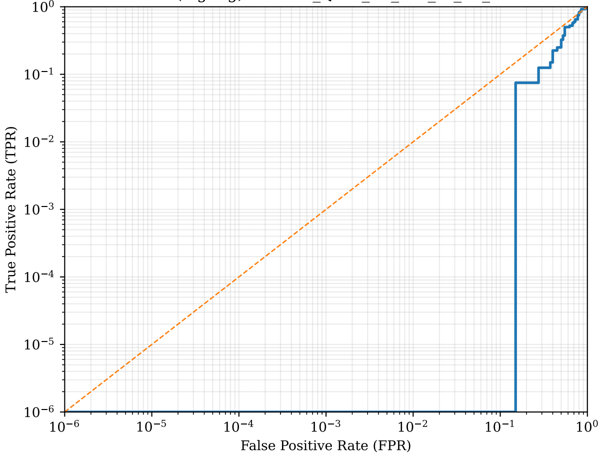
ROC (log-log): MNIST_QNN_eff_su2_r1_d6_s45
