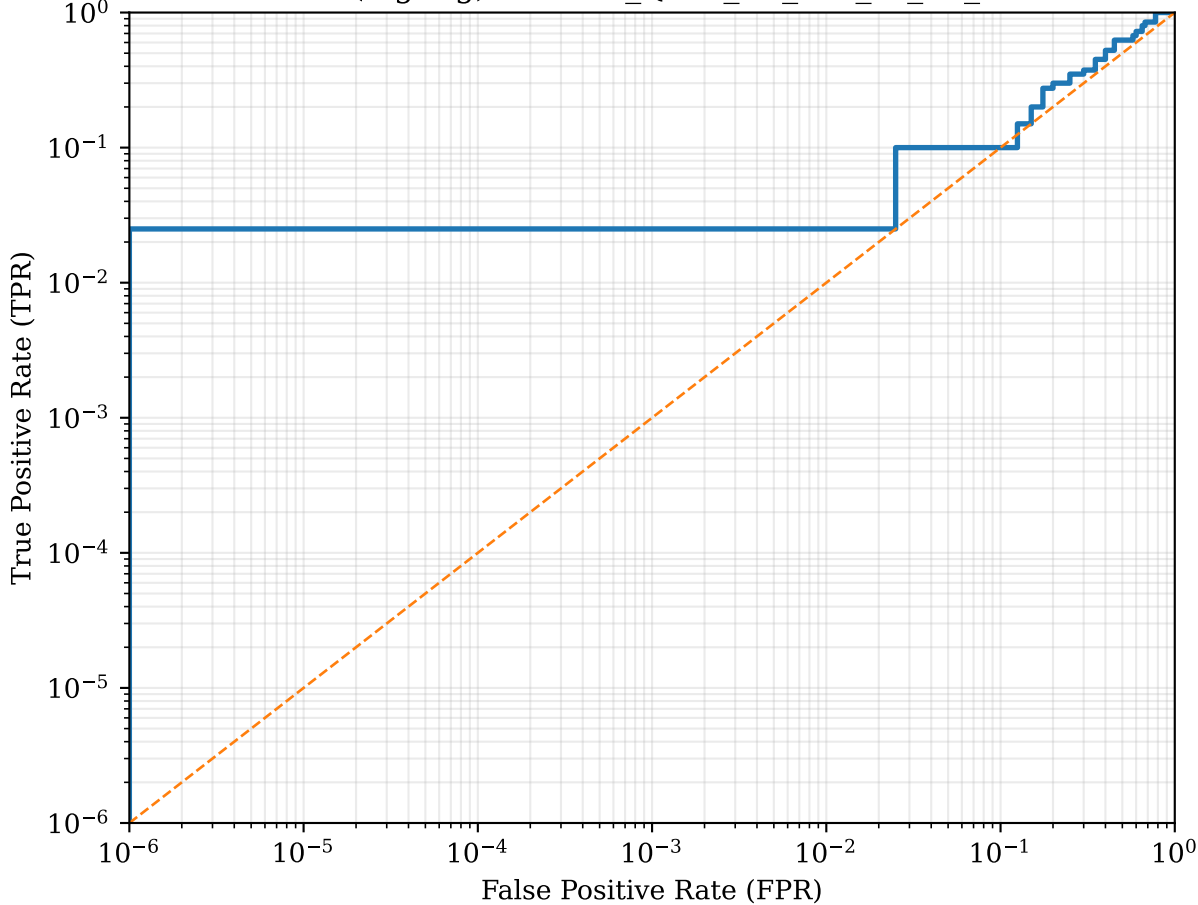
ROC (log-log): MNIST_QNN_eff_su2_r5_d6_s44
