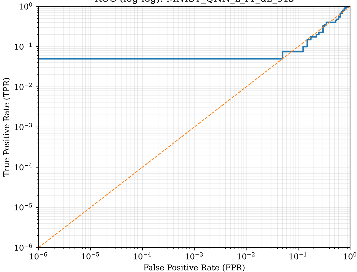
ROC (log-log): MNIST_QNN_z_r1_d2_s45
