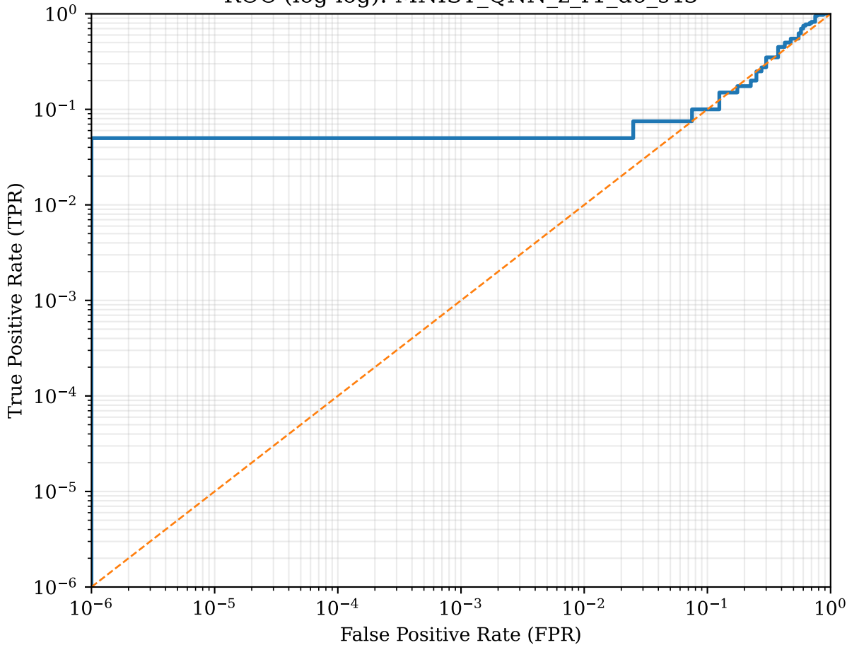
ROC (log-log): MNIST_QNN_z_r1_d6_s43
