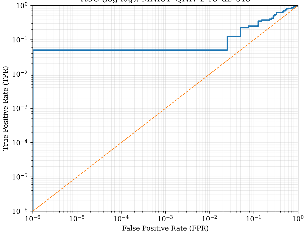
ROC (log-log): MNIST_QNN_z_r5_d2_s43
