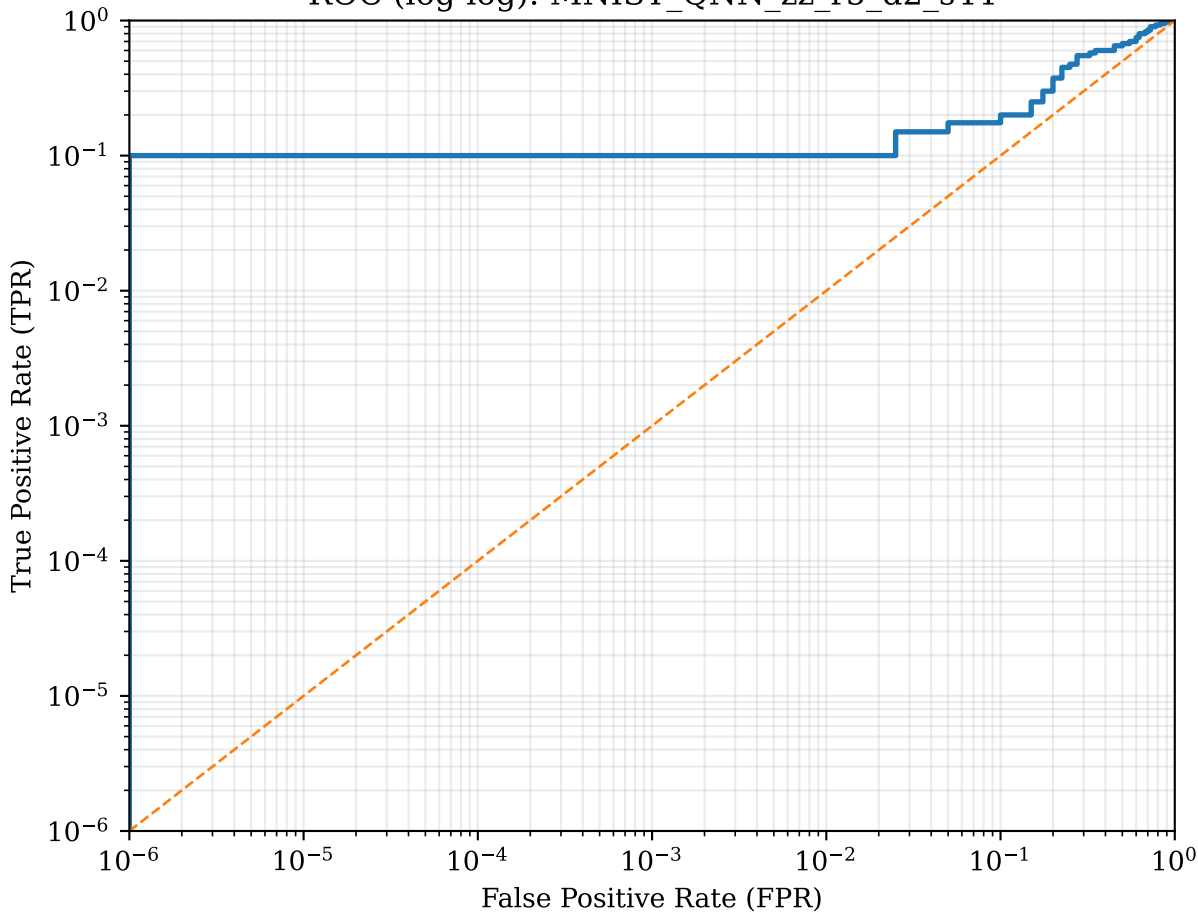
ROC (log-log): MNIST_QNN_zz_r5_d2_s44
