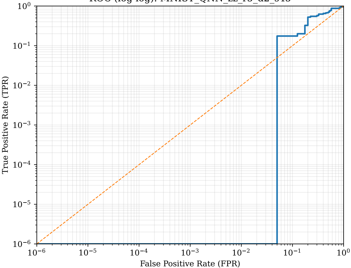
ROC (log-log): MNIST QNN zz r5 d2 s45
