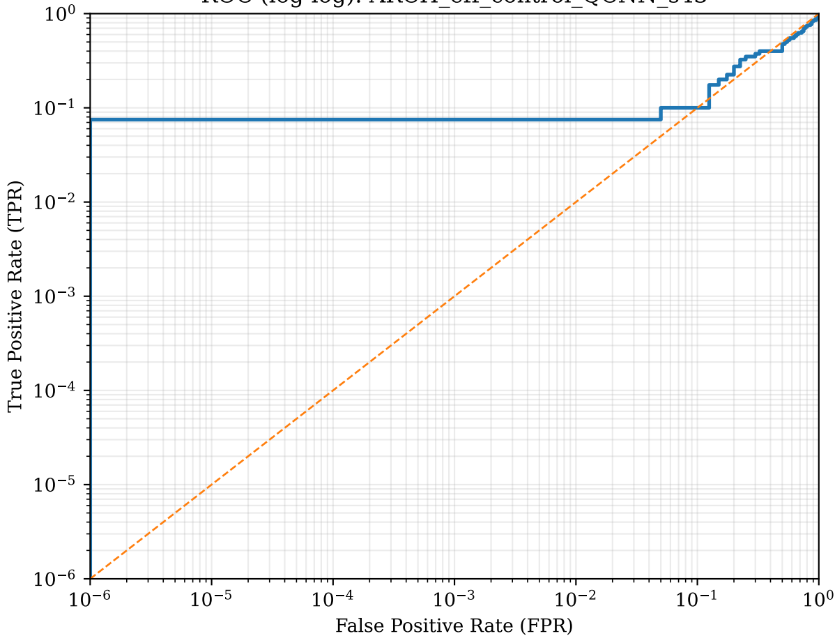
ROC (log-log): ARCH_eff_control_QCNN_s43
