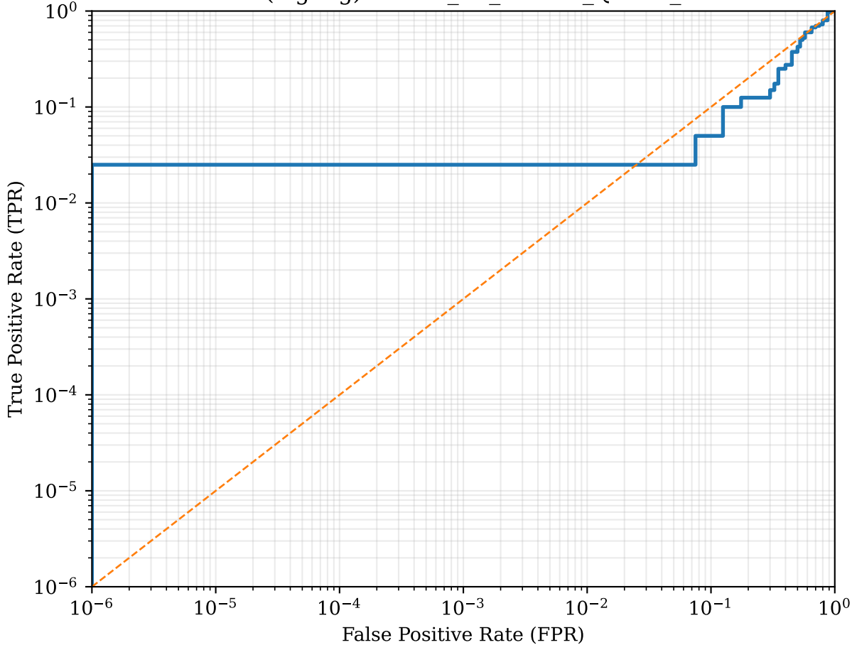
ROC (log-log): ARCH_eff_control_QCNN_s44
