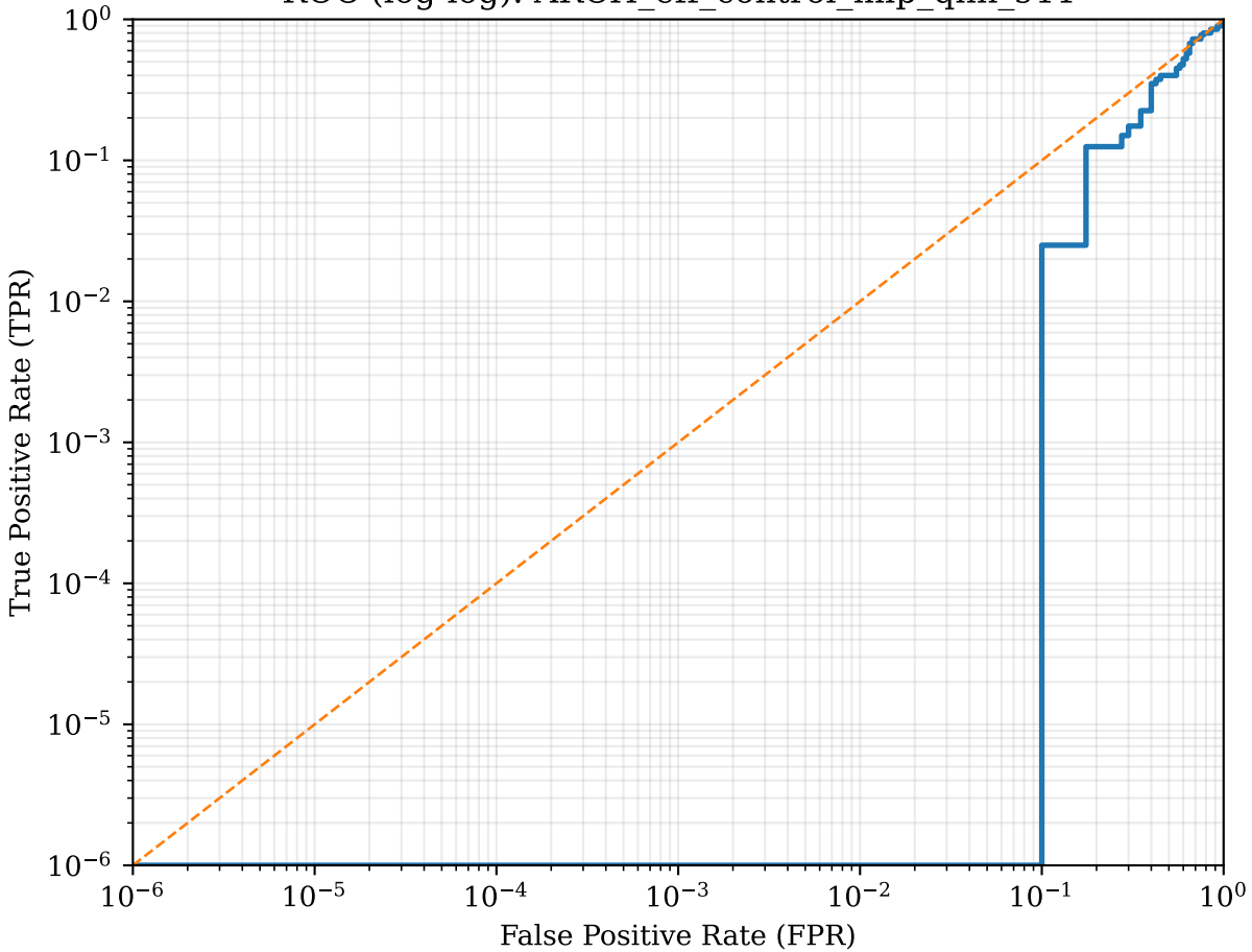
ROC (log-log): ARCH_eff_control_mlp_qnn_s44
