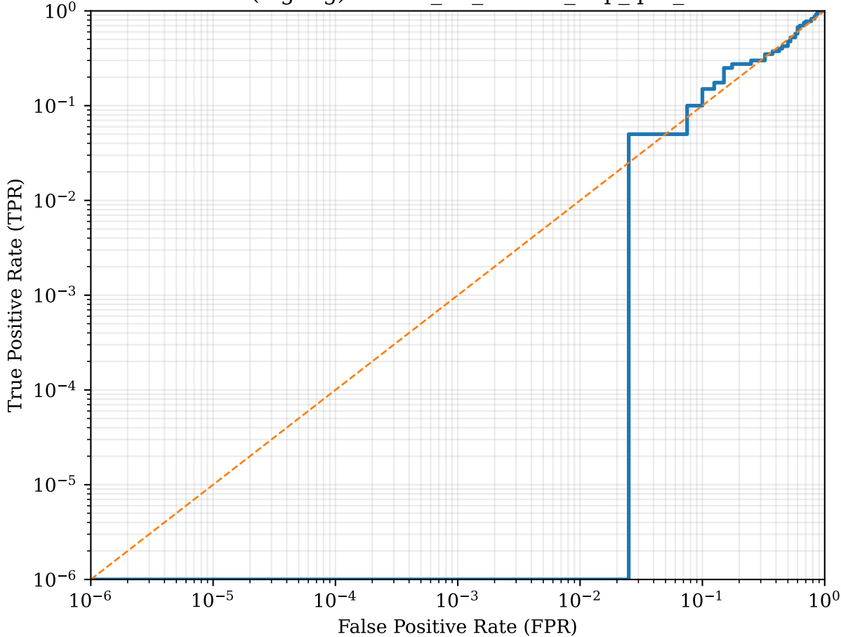
ROC (log-log): ARCH_eff_control_mlp_qnn_s45
