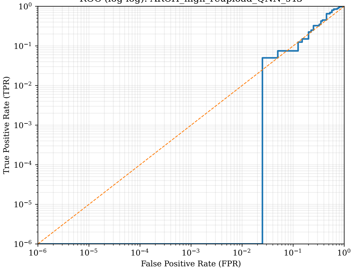
ROC (log-log): ARCH_high_reupload_QNN_s43
