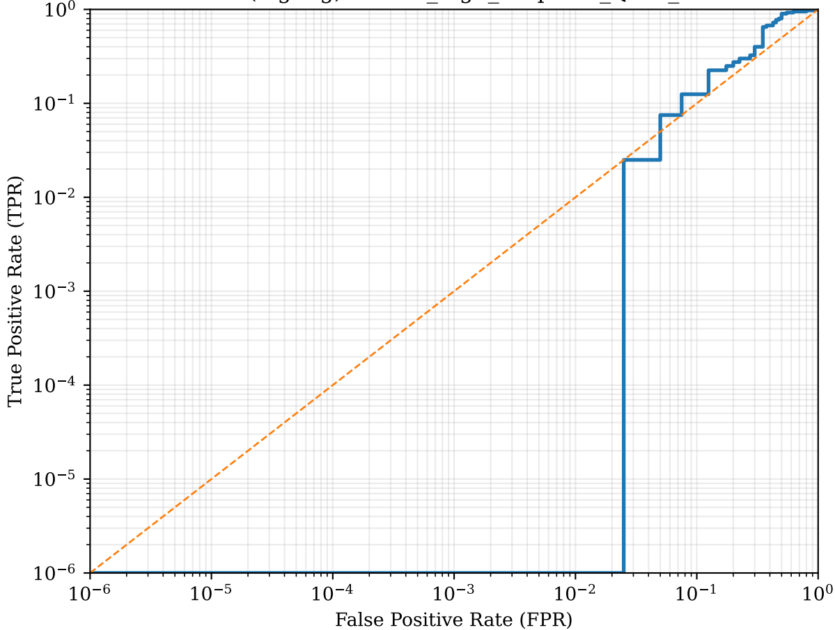
ROC (log-log): ARCH_high_reupload_QNN_s45
