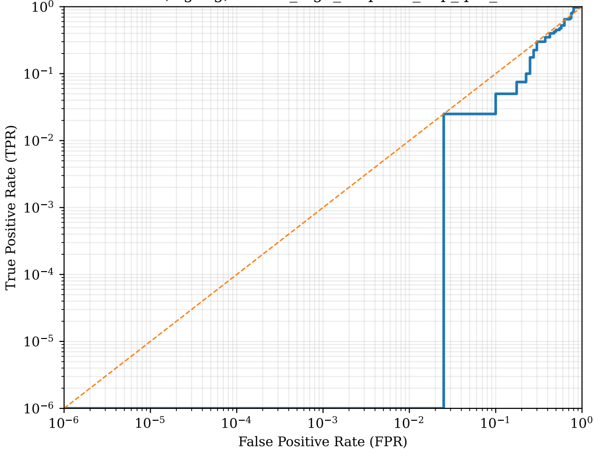
ROC (log-log): ARCH_high_reupload_mlp_qnn_s43
