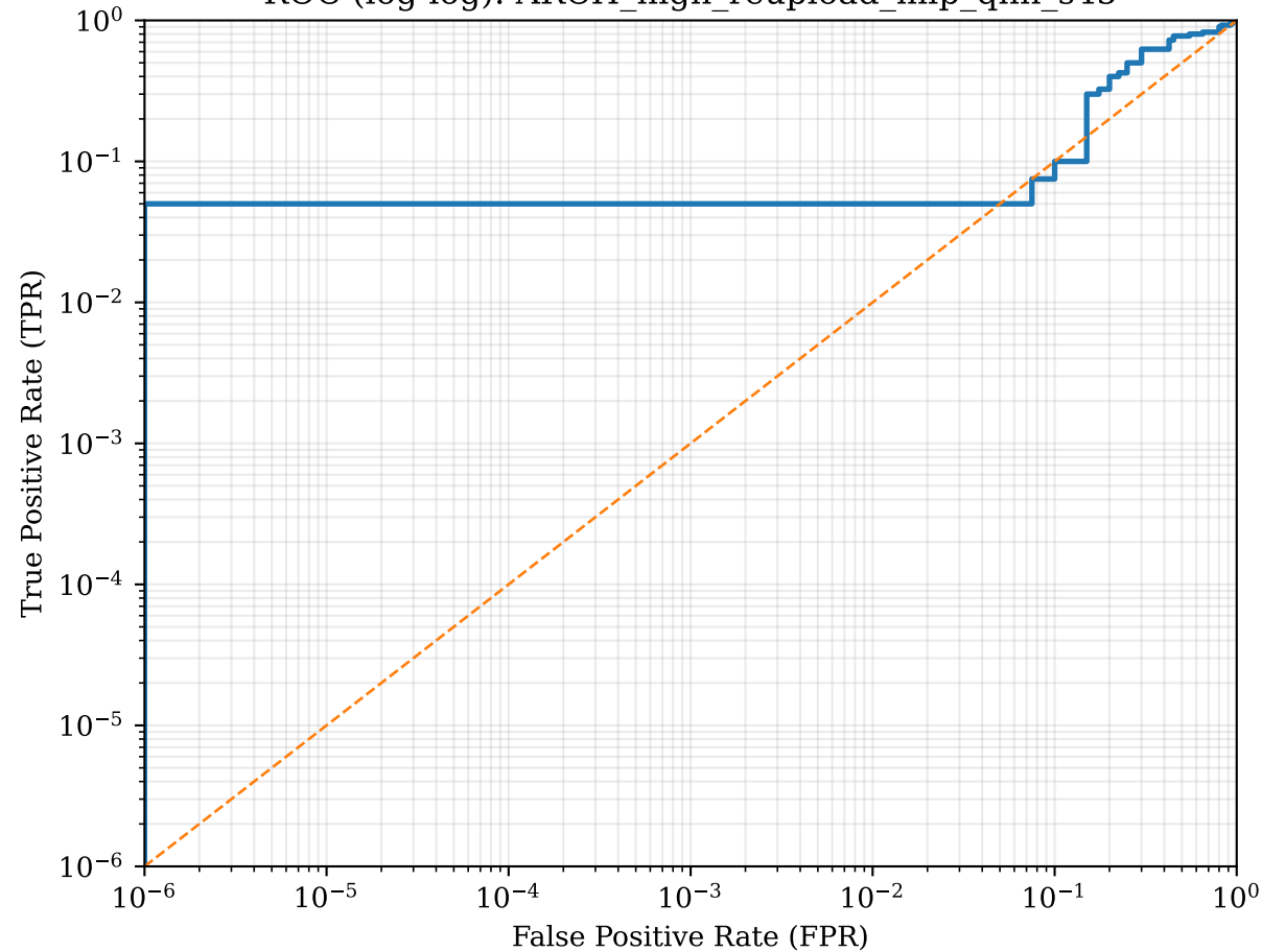
ROC (log-log): ARCH_high_reupload_mlp_qnn_s45
