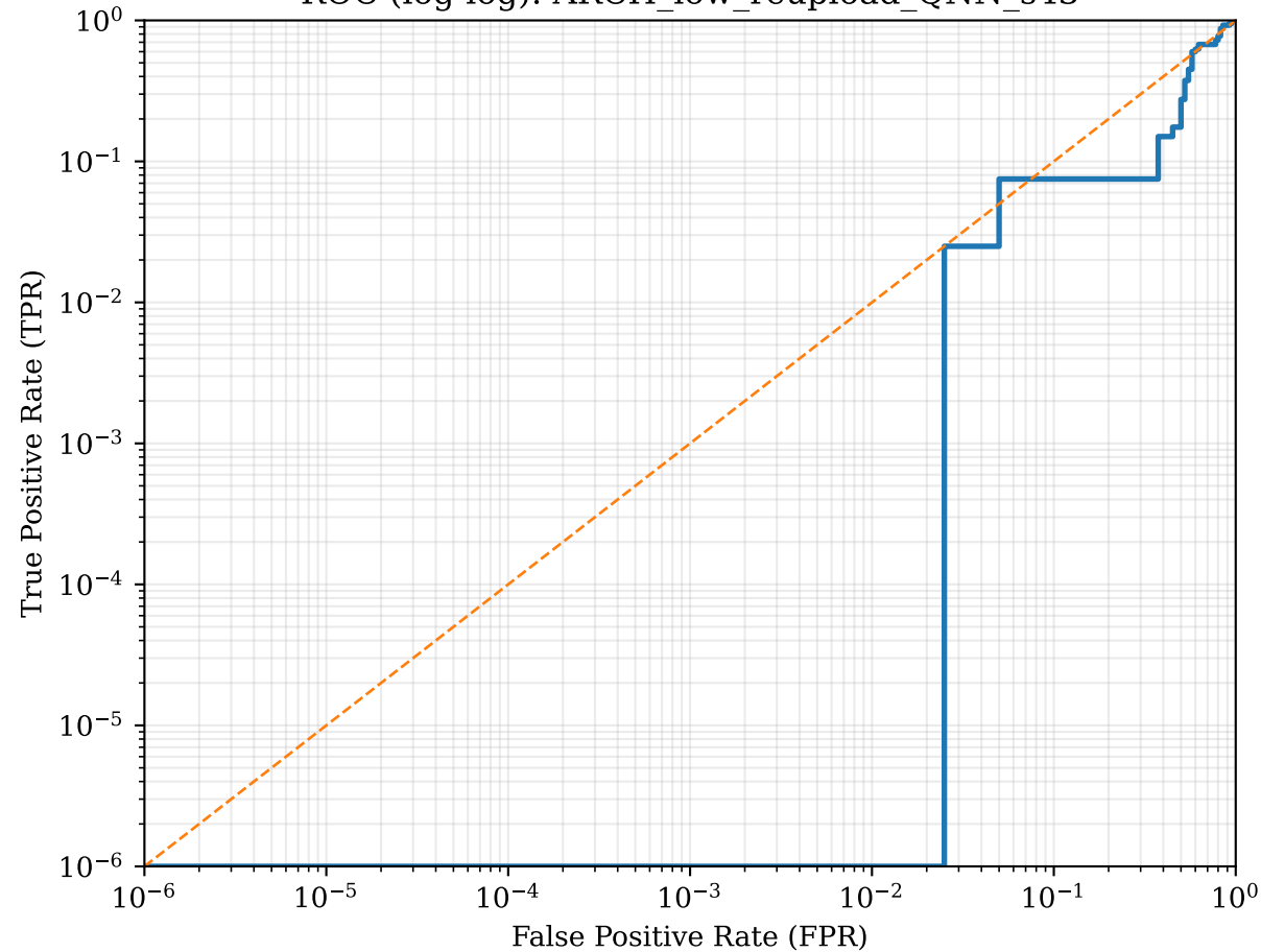
ROC (log-log): ARCH_low_reupload_QNN_s43
