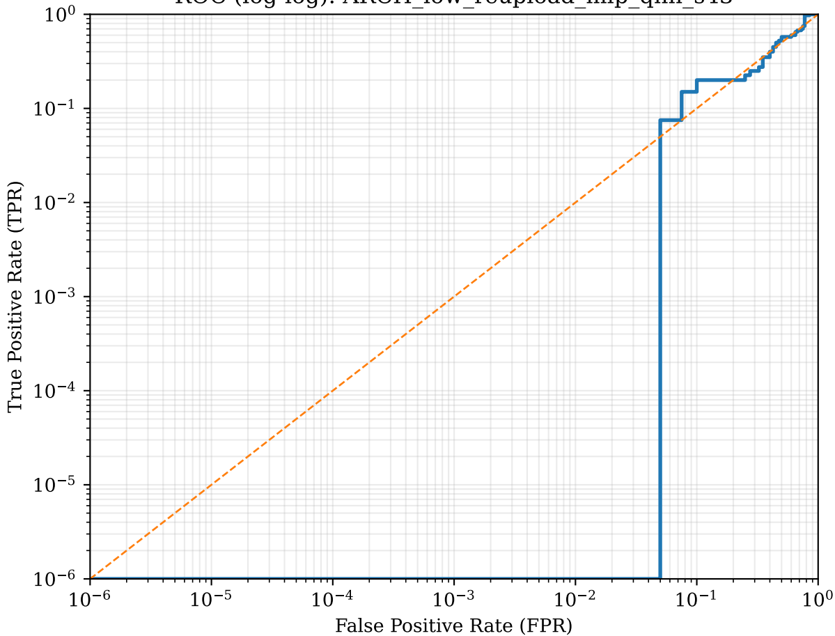
ROC (log-log): ARCH_low_reupload_mlp_qnn_s43
