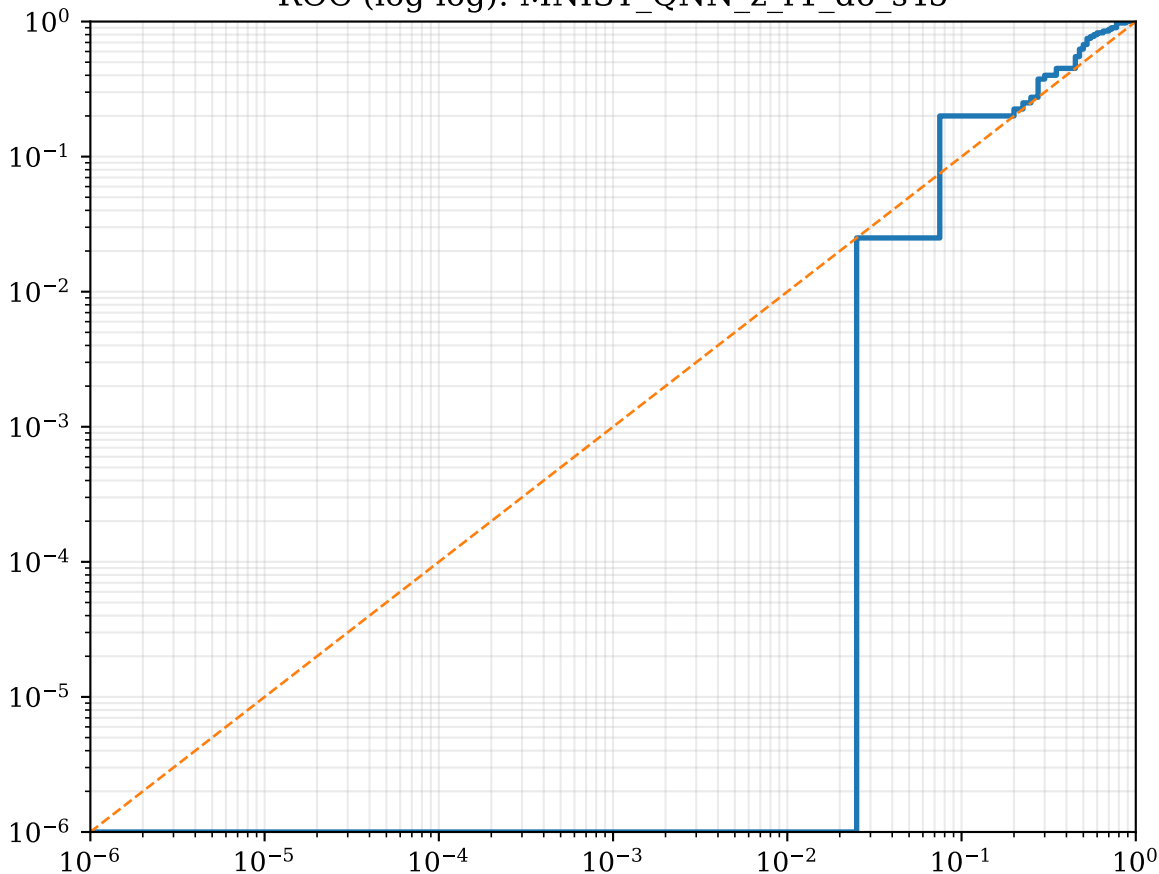
ROC (log-log): MNIST_QNN_z_r1_d6_s45
