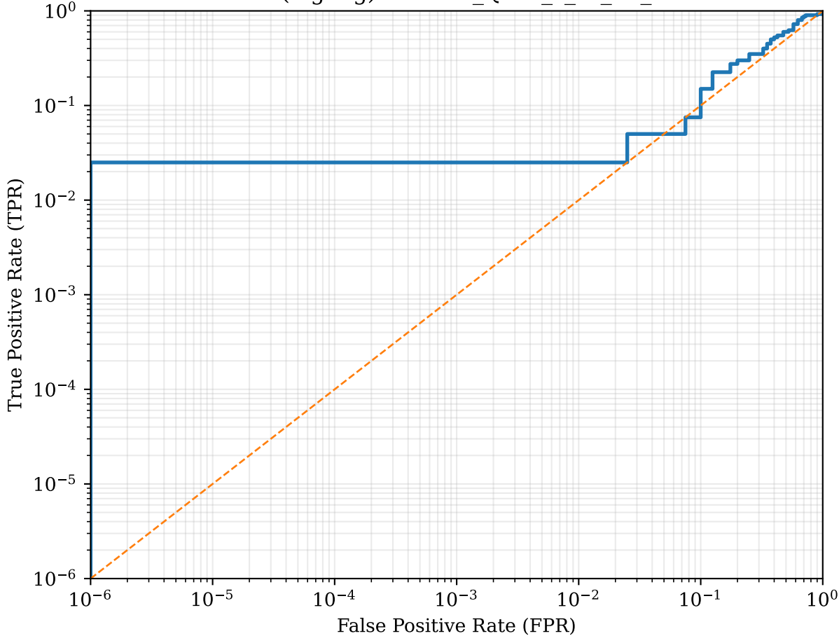
ROC (log-log): MNIST_QNN_z_r5_d2_s44
