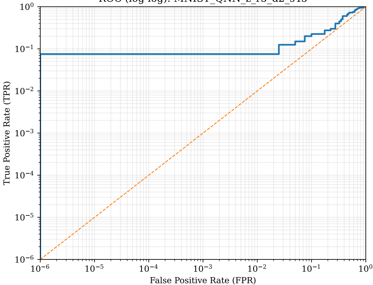
ROC (log-log): MNIST_QNN_z_r5_d2_s45
