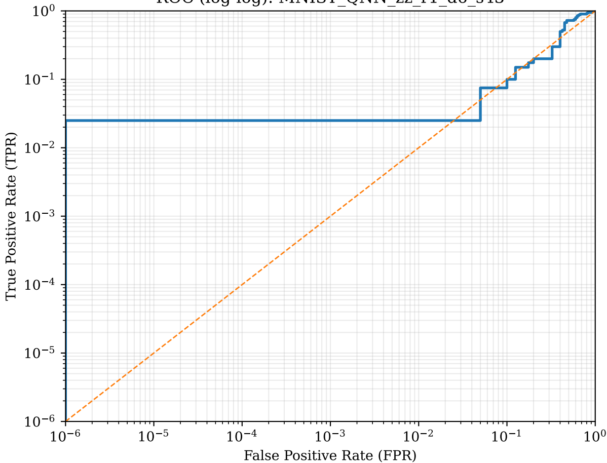
ROC (log-log): MNIST_QNN_zz_r1_d6_s43
