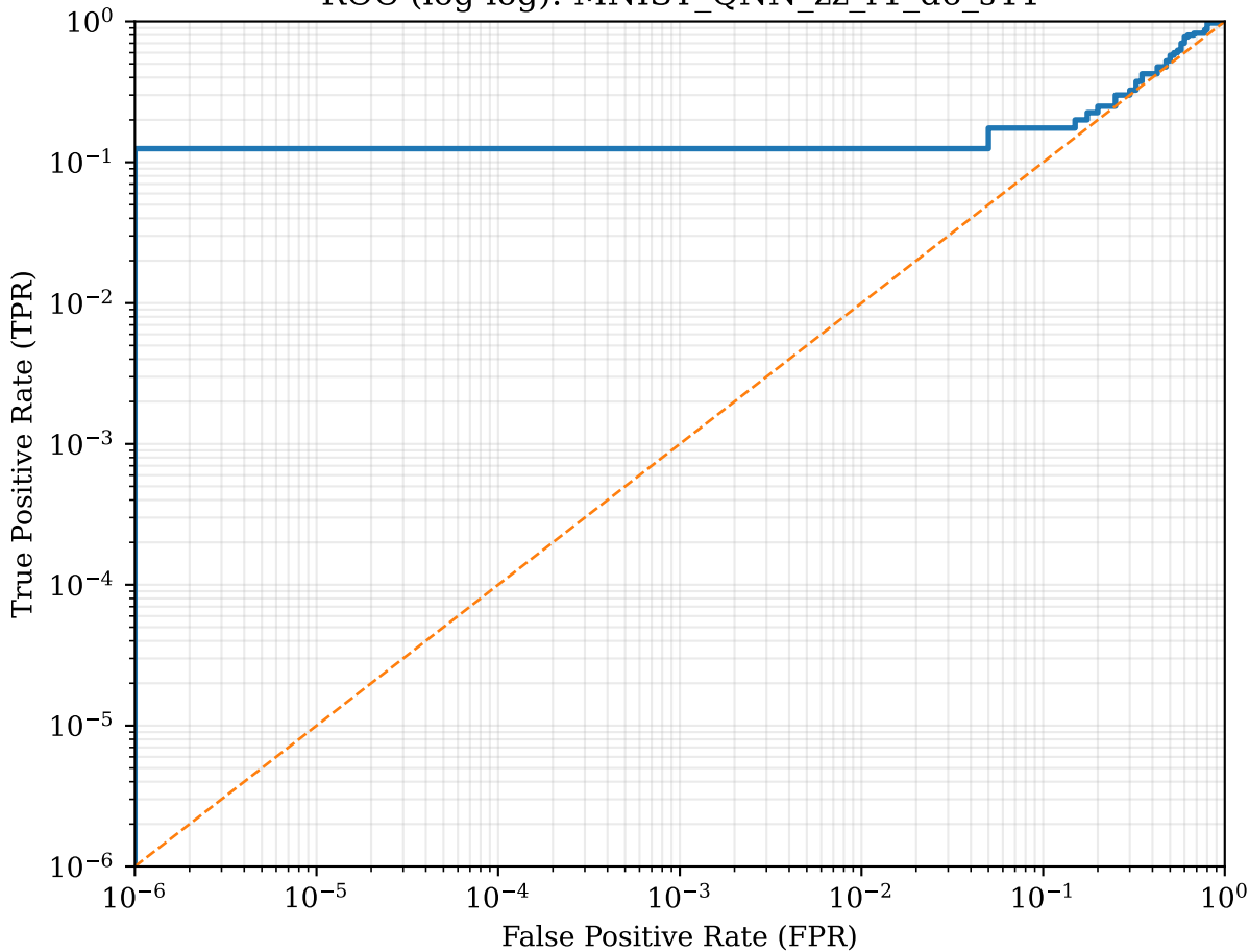
ROC (log-log): MNIST_QNN_zz_r1_d6_s44
