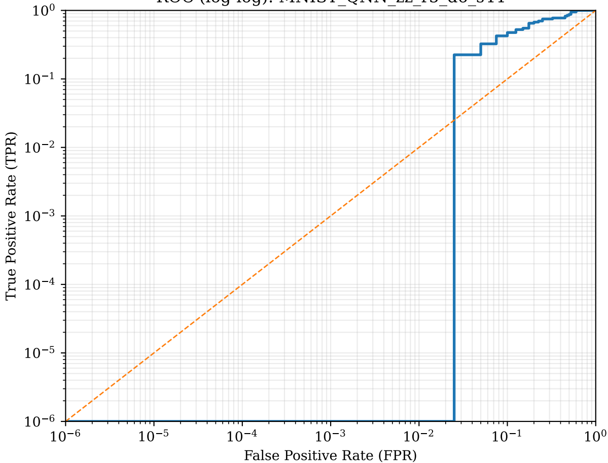
ROC (log-log): MNIST_QNN_zz_r5_d6_s44
