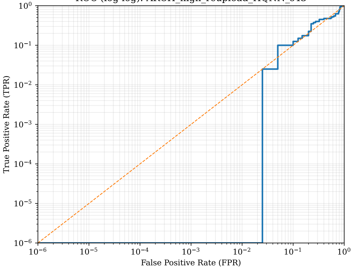
ROC (log-log): ARCH_high_reupload_HQNN_s43
