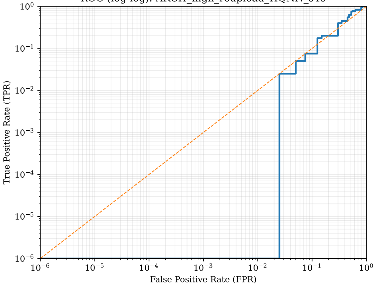
ROC (log-log): ARCH_high_reupload_HQNN_s45
