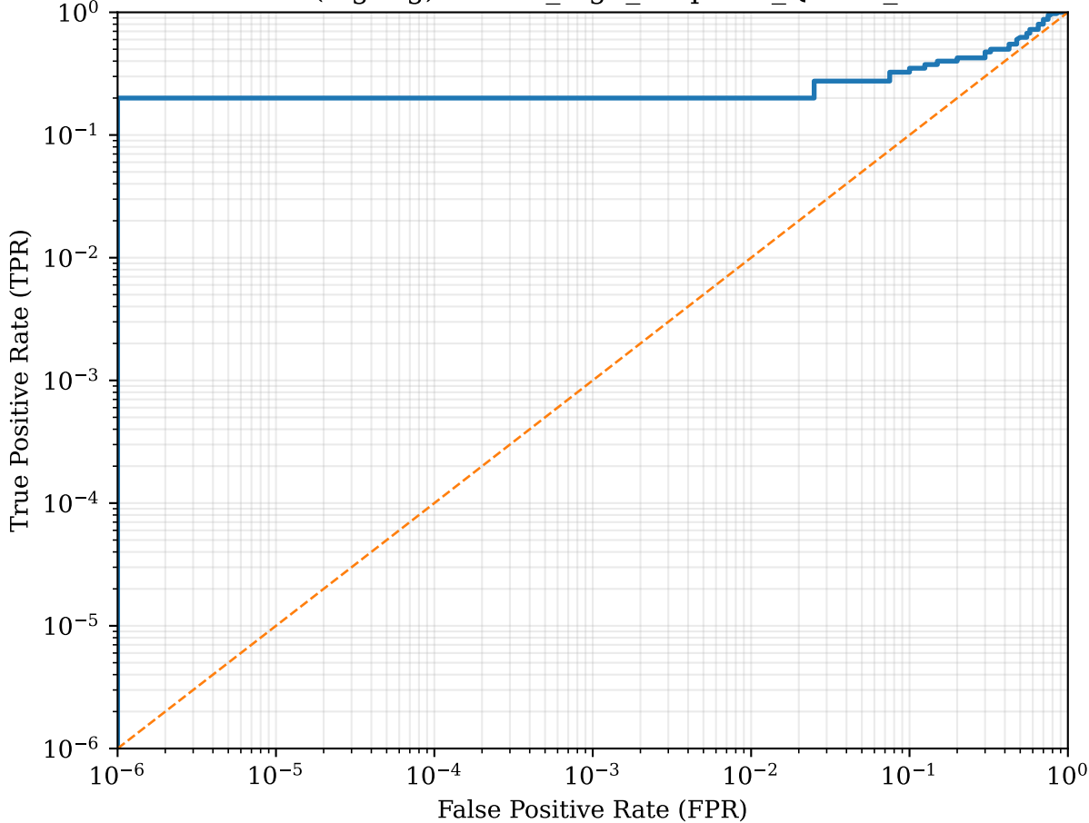
ROC (log-log): ARCH_high_reupload_QCNN_s43
