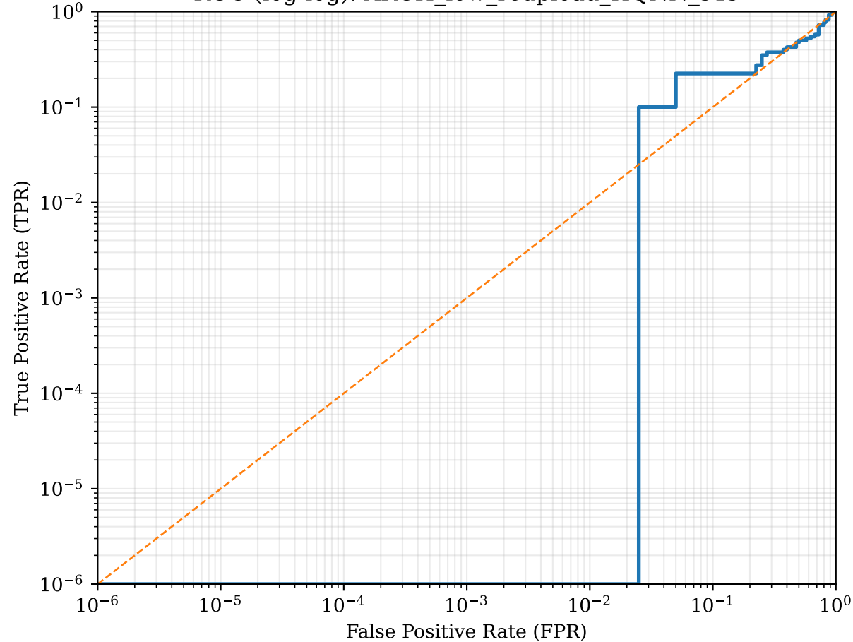
ROC (log-log): ARCH_low_reupload_HQNN_s45
