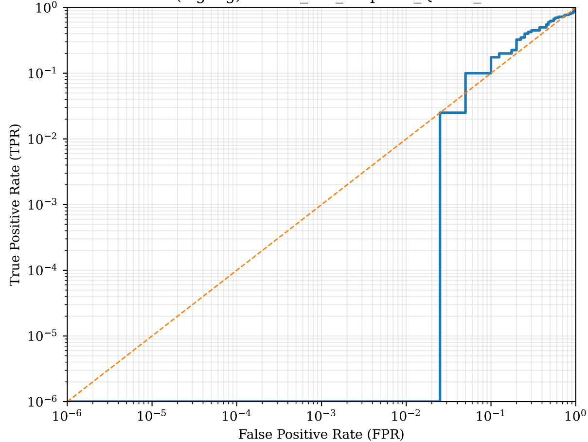
ROC (log-log): ARCH_low_reupload_QCNN_s43
