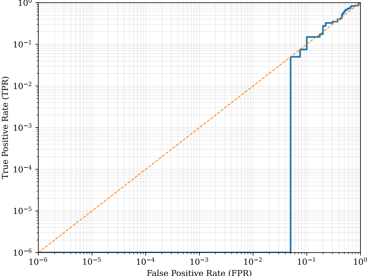
ROC (log-log): MNIST QNN eff su2 r1 d2 s44
