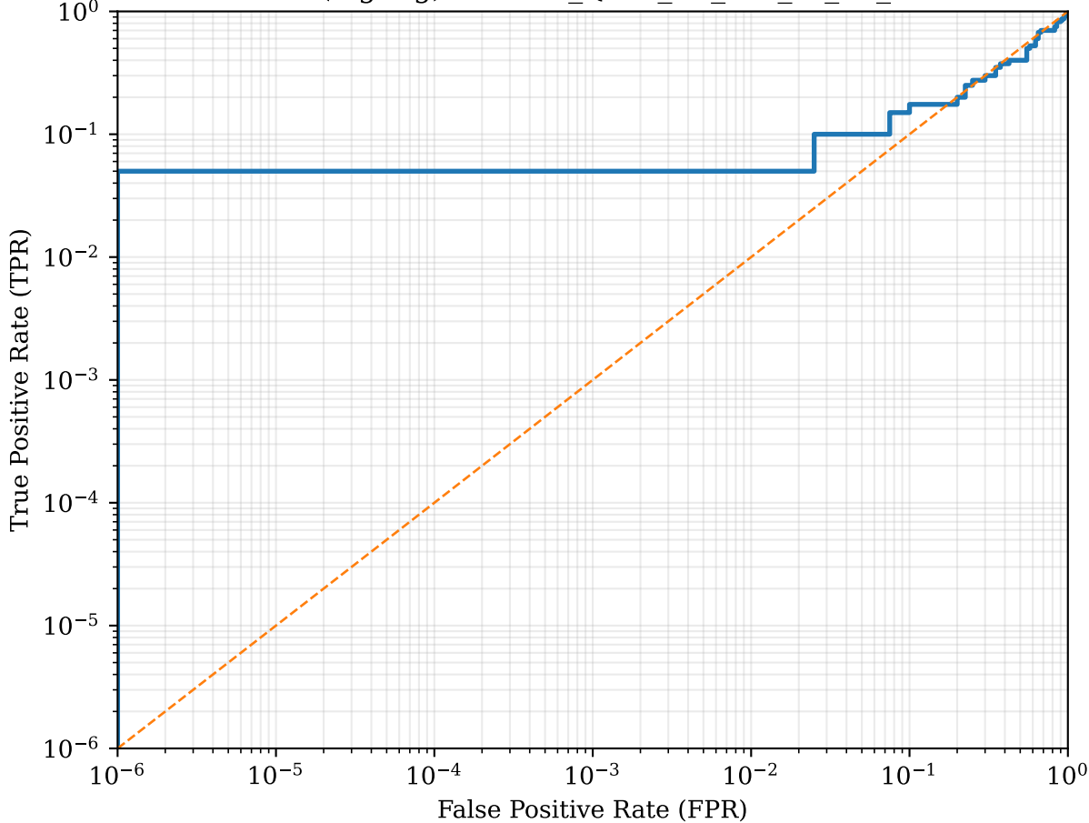
ROC (log-log): MNIST_QNN_eff_su2_r1_d6_s43
