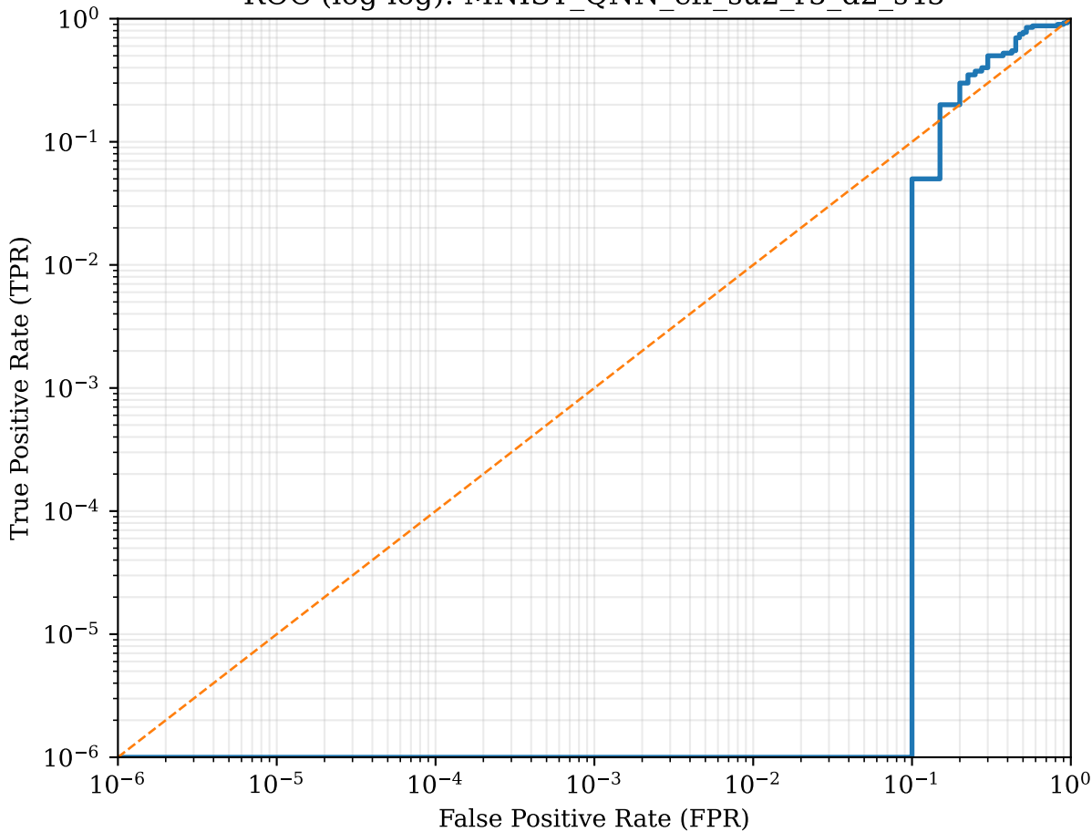
ROC (log-log): MNIST_QNN_eff_su2_r5_d2_s45
